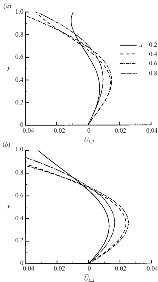
FIGURE 12. The O(\Delta^2) steady Lagrangian axial drift velocities (a) and (b) corresponding to figures 11(a) and 11(b), respectively.
