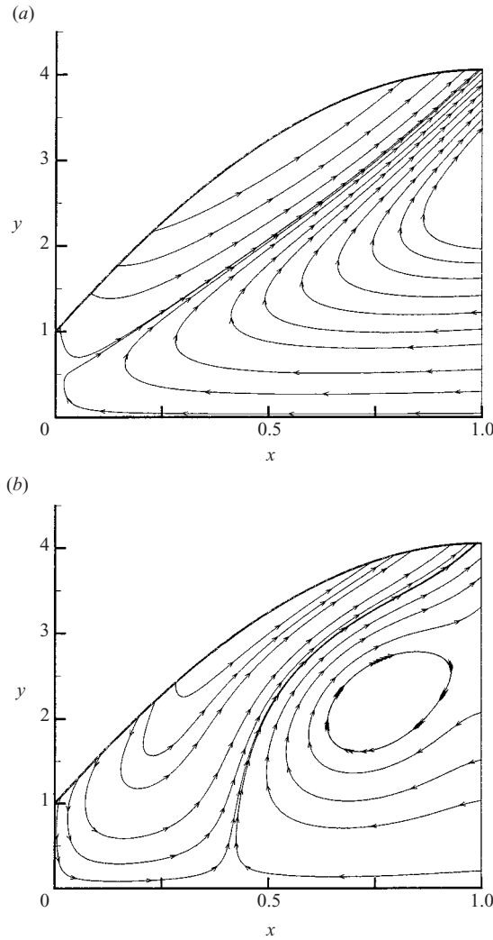
FIGURE 14. The O(\Delta^2) cycle-averaged streamlines. (a) Insoluble case with \hat{C}a = 1 , M = 1 , Ps = 10 , V_0 = 3 . (b) Soluble case with \hat{C}a = 1 , M = 1 , Ps = 10 , Pe_b = 1 , K = 1 , \beta = 0.1 , V_0 = 3 .
