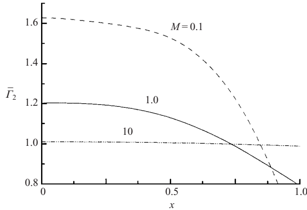
FIGURE 6. The O(\Delta^2) cycle-averaged surface concentration \bar{T}_2 versus x corresponding to figure 5. The rigid end (the extensible end) is at x=0 ( x=1 ). \bar{T}_2 is higher near the rigid end and decreases as it approaches the extensible end. The gradient of \bar{T}_2 diminishes as M increases.
